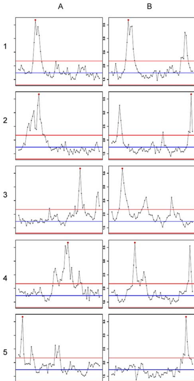
Figure 5. Examples of oligonucleotide probes from the “Operon (a)” probe set where T7 bias motifs are identified by plotting the rank related motif bias (Mr). Column A and B: Ten examples plots for probe sequences that contain the T7 primer 1 3' spacer motif CCTCC. The 70-mer probe sequence is split in 6-mer fragments over the x-axis and the intensity rank related motif bias (Mr) is plotted on the y-axis. The red dot represents the position of the CCTCC motif in the probe sequence. The blue line is the average over all the motifs from a probe sequence, the red lines represent the standard deviation up and down for the same measurement over all 6-mers in the whole probe. Operon Ids for the probes listed A1 to B5 and C1 to D5: H200018976, H300020020, H200016156, H300007790, H300013997, H300022725, H200010013, H300019787, H200001204, H200004220. doi:10.1371/journal.pone.0001980.g005
